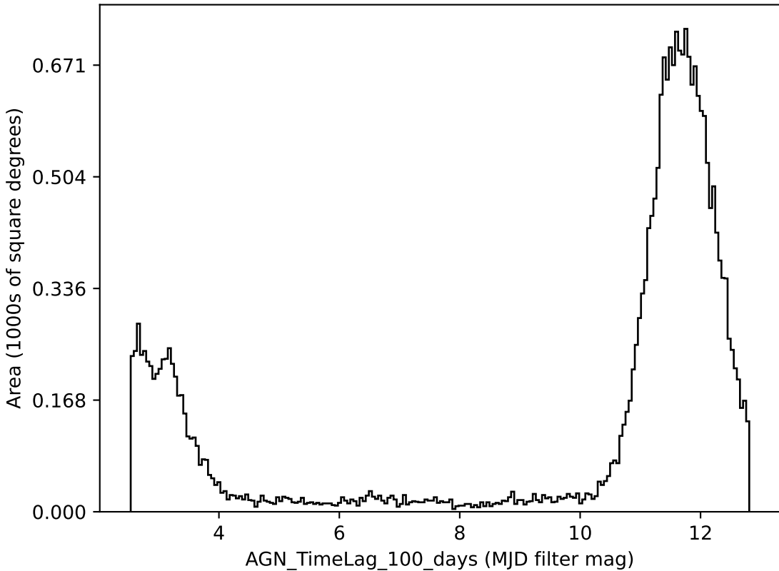
early_u_fpextra4.0_v3.4_10yrs all bands: AGN_TimeLag_100_days
