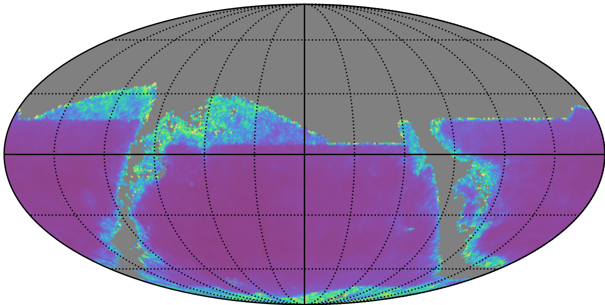
early_u_fpextra4.0_v3.4_10yrs z band: AGN SF_uncert
