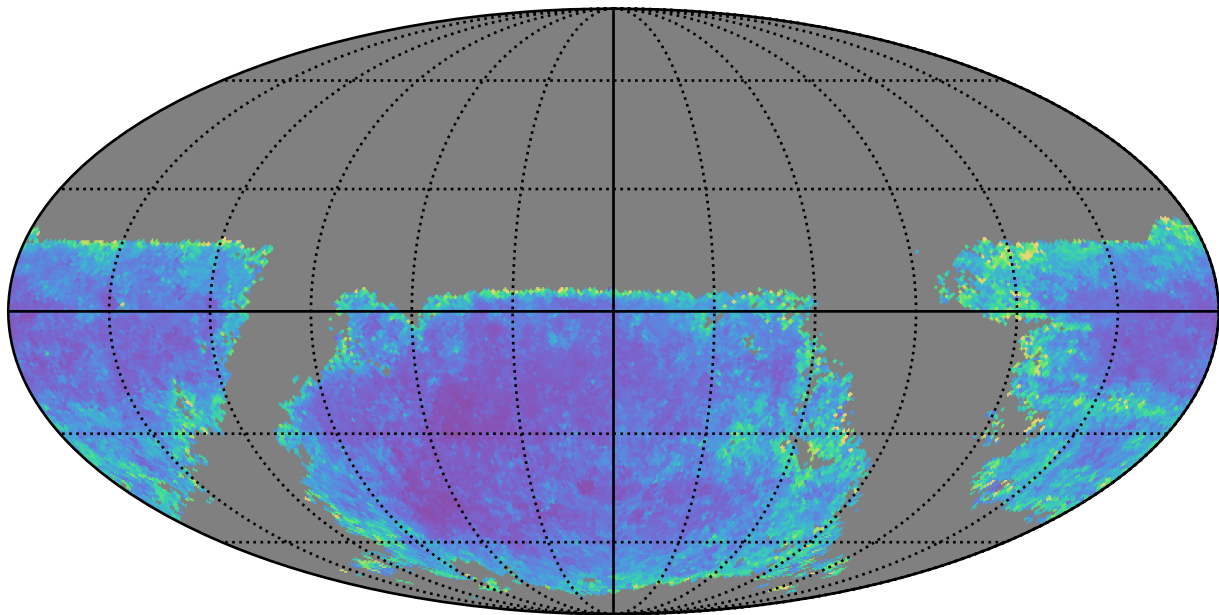
early_u_fpextra4.0_v3.4_10yrs u band: AGN SF_uncert
