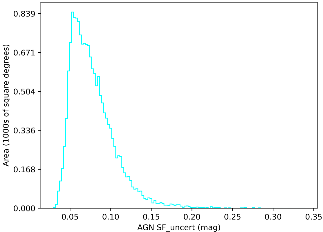
early_u_fpextra4.0_v3.4_10yrs u band: AGN SF_uncert
