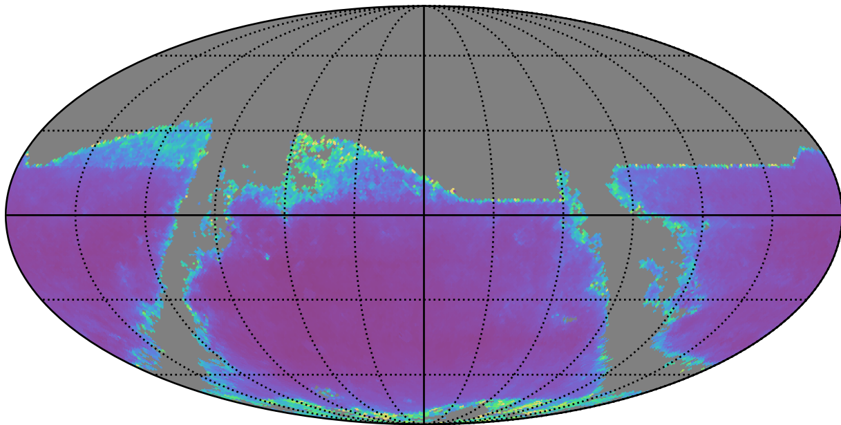
early_u_fpextra4.0_v3.4_10yrs r band: AGN SF_uncert
