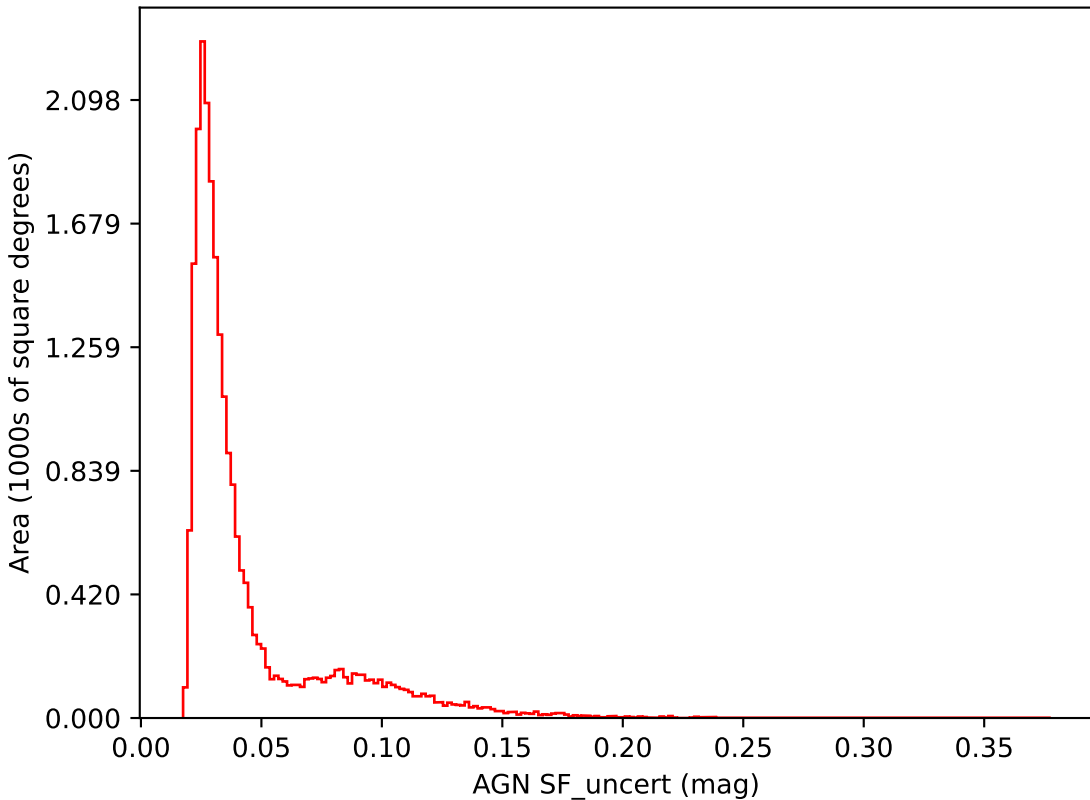
early_u_fpextra4.0_v3.4_10yrs i band: AGN SF_uncert
