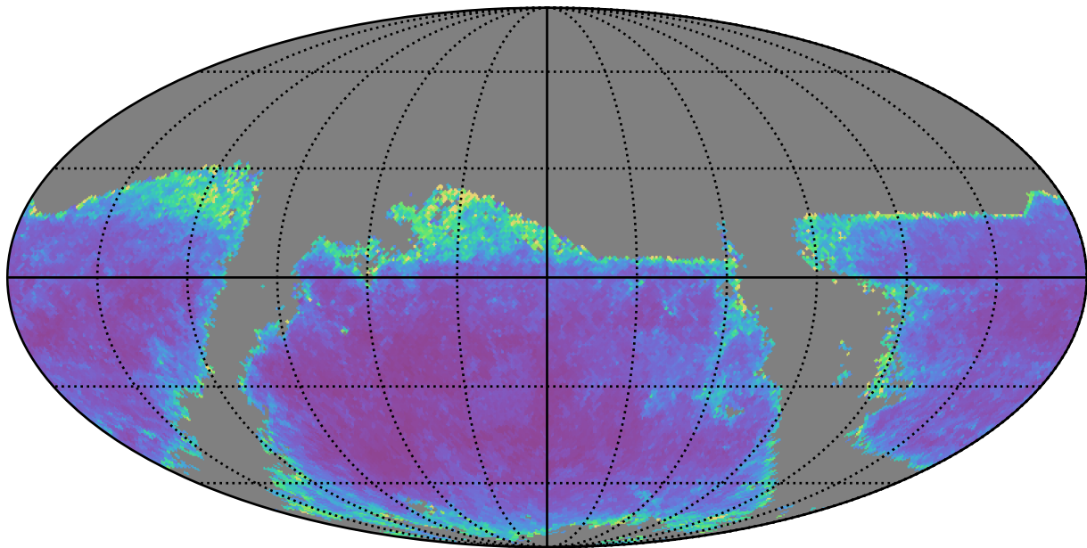
early_u_fpextra4.0_v3.4_10yrs g band: AGN SF_uncert
