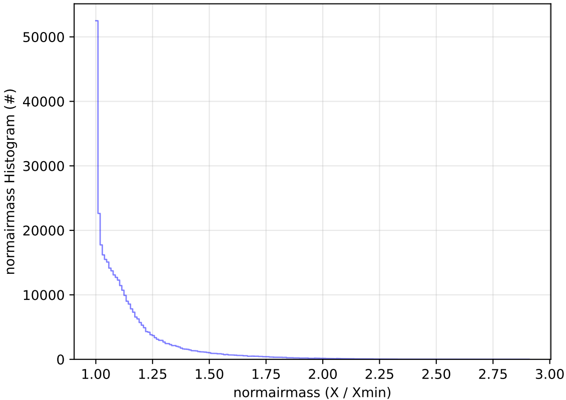
early_u_fpextra4.0_v3.4_10yrs WFD y band: normairmass Histogram
