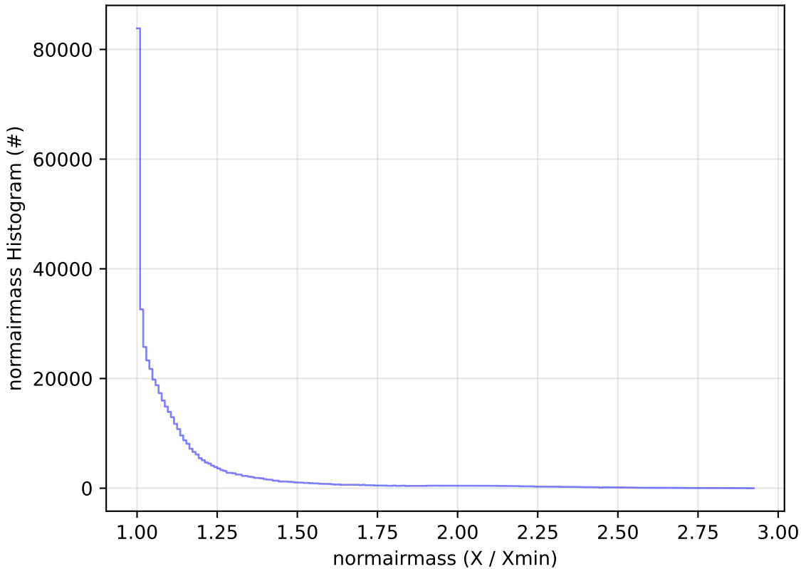
early_u_fpextra4.0_v3.4_10yrs WFD i band: normairmass Histogram
