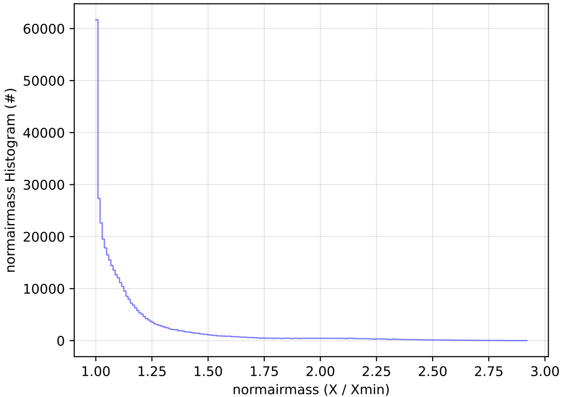
early_u_fpextra4.0_v3.4_10yrs All sky z band: normairmass Histogram
