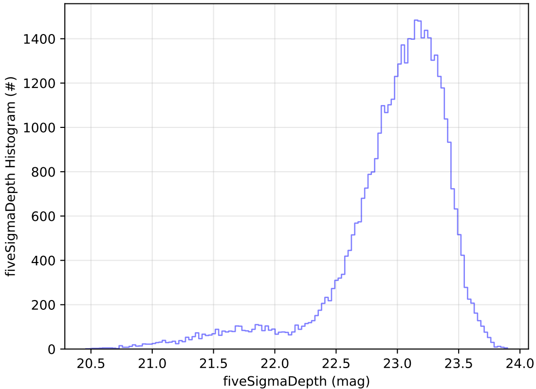
early_u_fpextra4.0_v3.4_10yrs Yr 1 z band: fiveSigmaDepth Histogram
