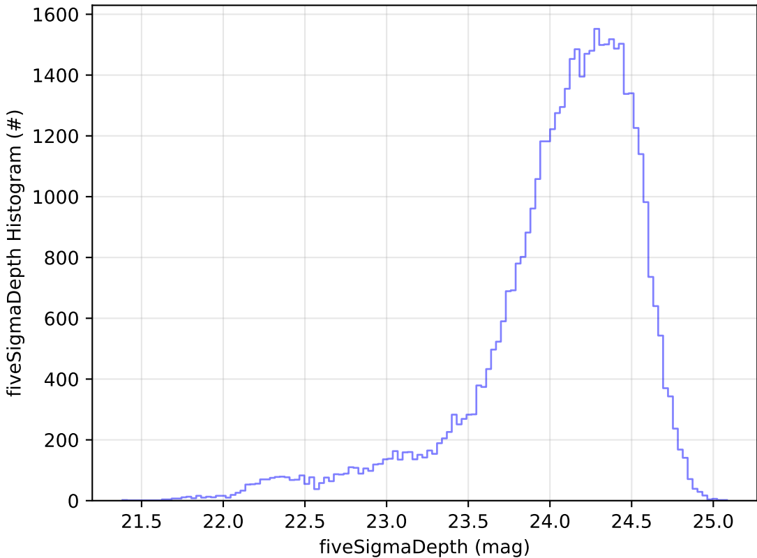
early_u_fpextra4.0_v3.4_10yrs Yr 1 r band: fiveSigmaDepth Histogram
