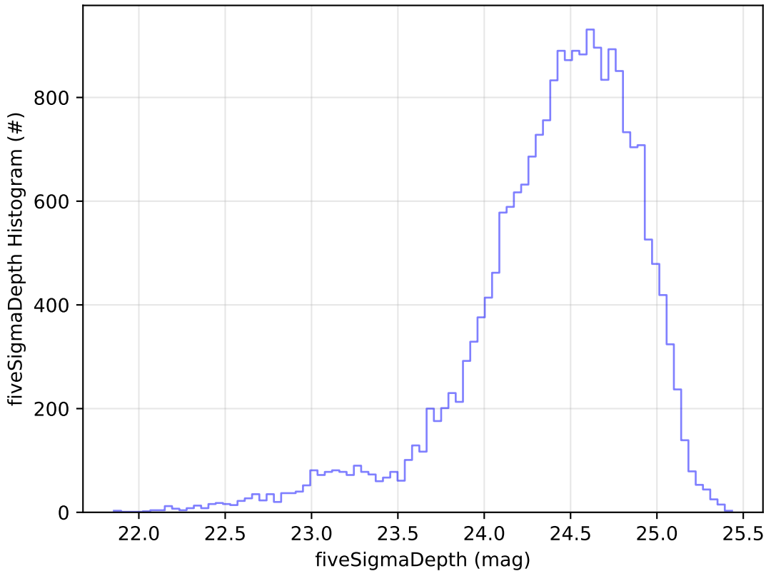
early_u_fpextra4.0_v3.4_10yrs Yr 1 g band: fiveSigmaDepth Histogram
