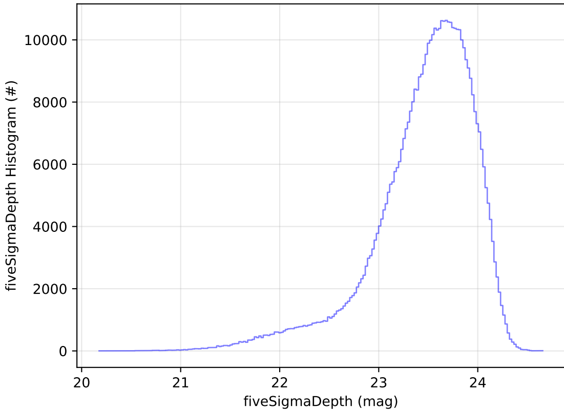
early_u_fpextra4.0_v3.4_10yrs WFD i band: fiveSigmaDepth Histogram
