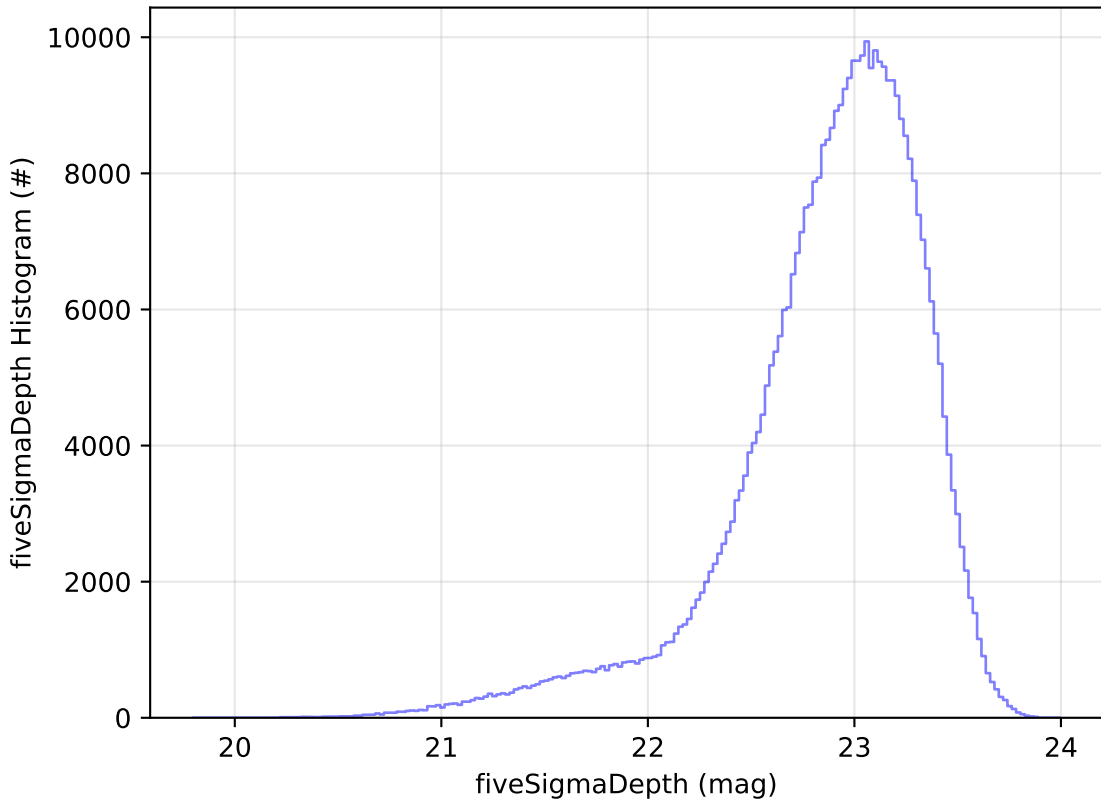
early_u_fpextra4.0_v3.4_10yrs All sky z band: fiveSigmaDepth Histogram
