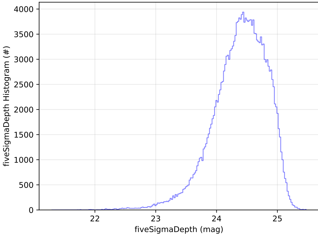
early_u_fpextra4.0_v3.4_10yrs All sky g band: fiveSigmaDepth Histogram
