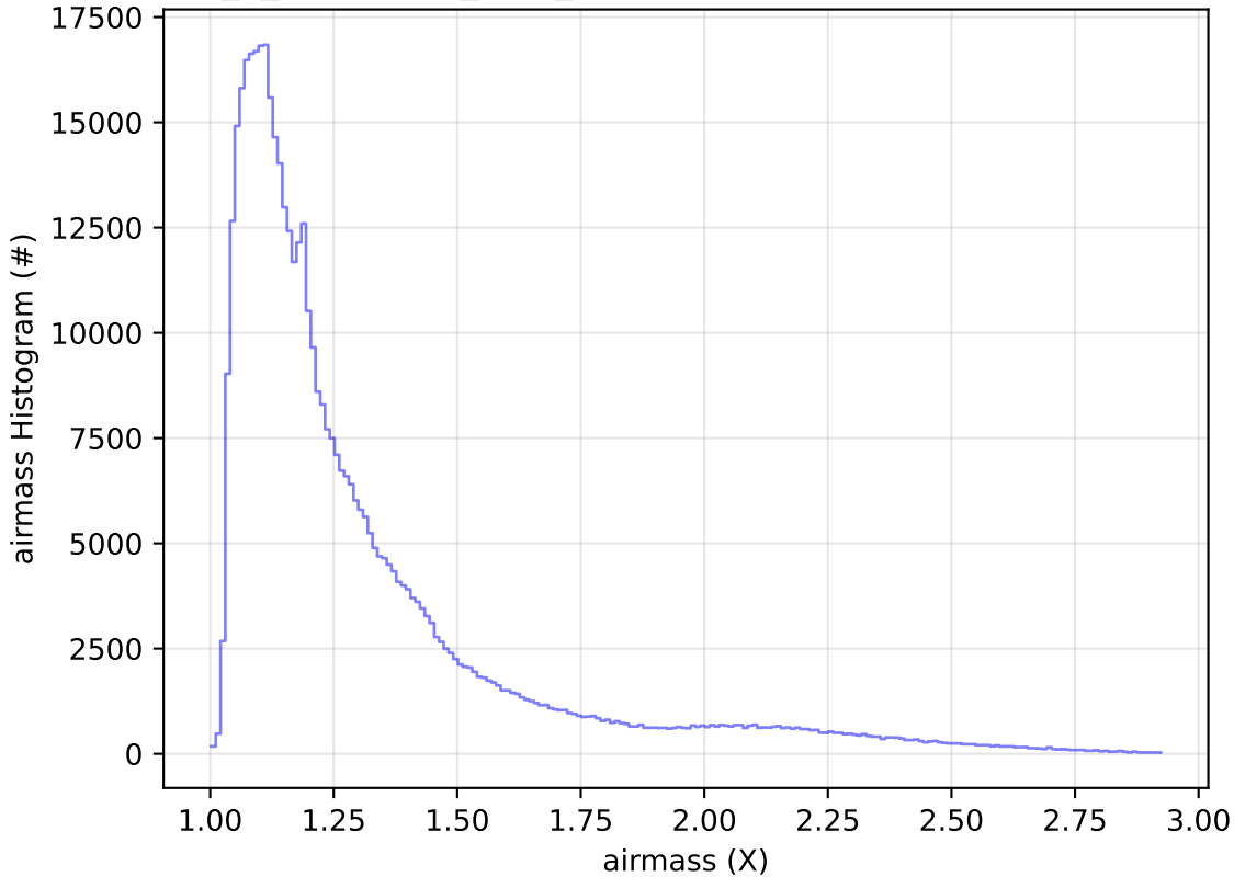
early_u_fpextra4.0_v3.4_10yrs WFD i band: airmass Histogram
