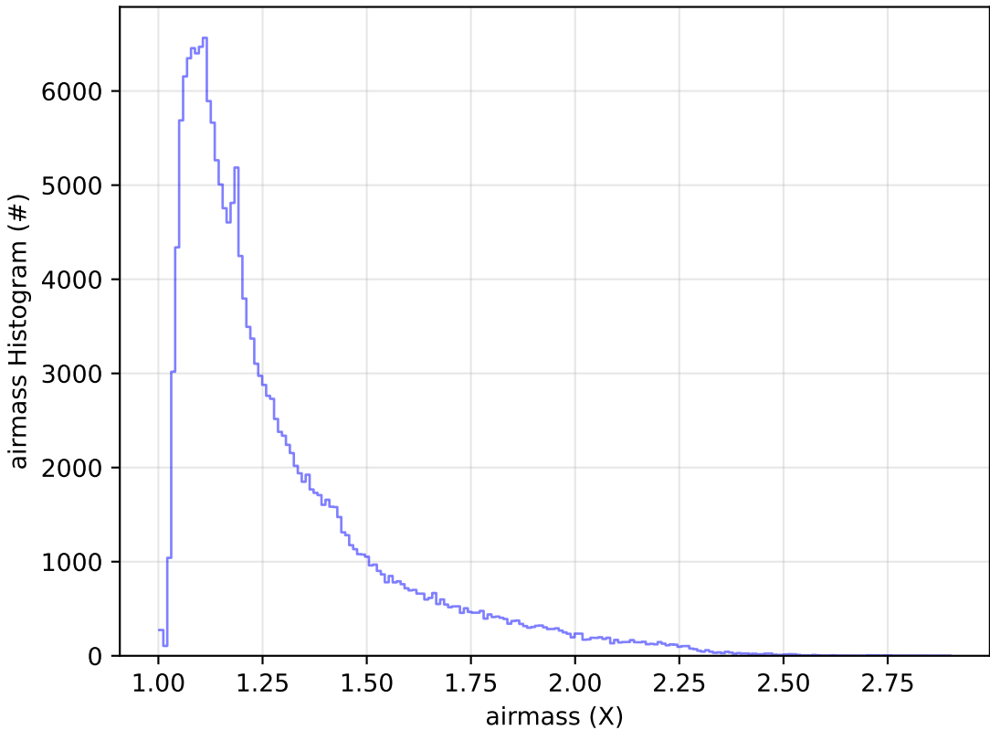
early_u_fpextra4.0_v3.4_10yrs WFD g band: airmass Histogram
