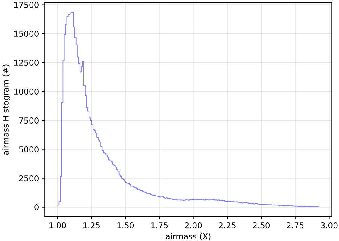
early_u_fpextra4.0_v3.4_10yrs All sky i band: airmass Histogram
