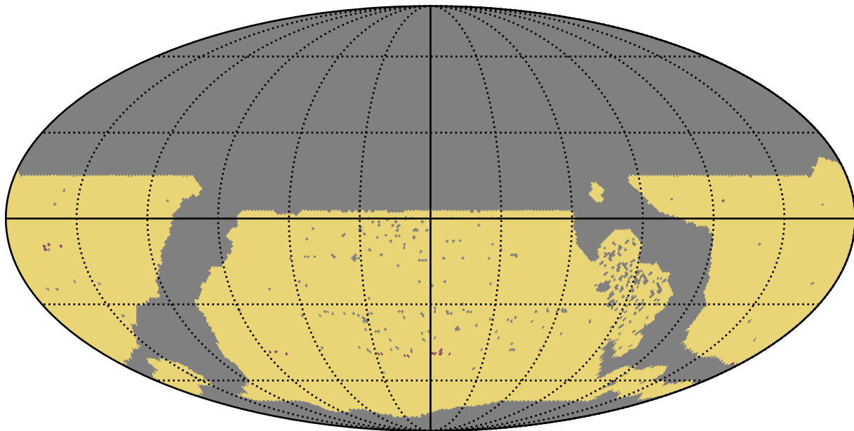
early_u_fpextra4.0_v3.4_10yrs WFD: RapidRevisits
