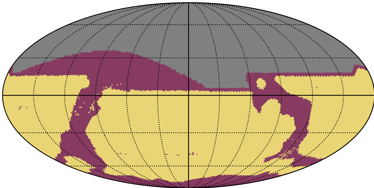
early_u_fpextra4.0_v3.4_10yrs All sky: RapidRevisits
