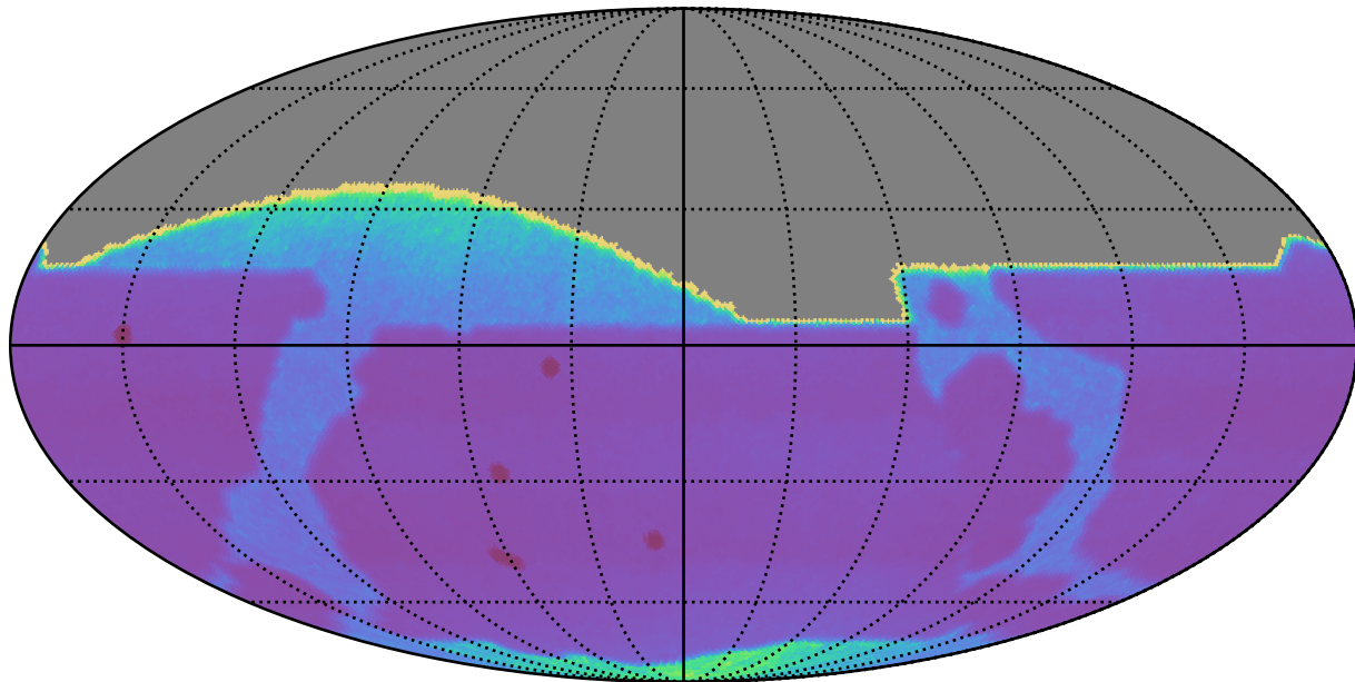
early_u_fpextra4.0_v3.4_10yrs All sky: Proper Motion Uncert @ 20.5
