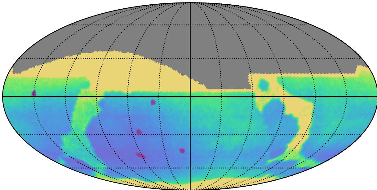
early_u_fpextra4.0_v3.4_10yrs All sky: Parallax Uncert @ 24.0
