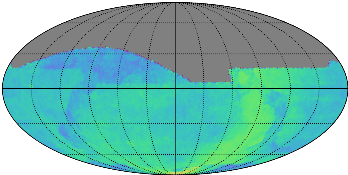
early_u_fpextra4.0_v3.4_10yrs All sky: Parallax Coverage @ 24.0
