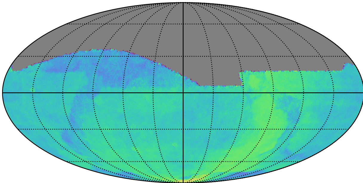
early_u_fpextra4.0_v3.4_10yrs All sky: Parallax Coverage @ 22.4
