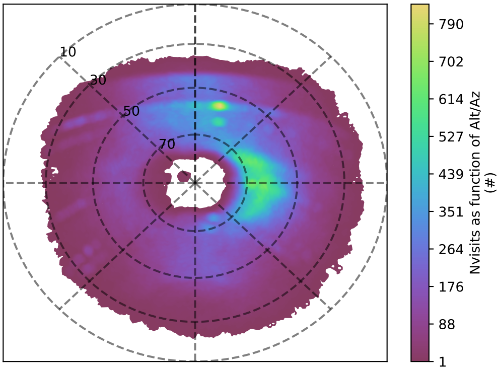
early_u_fpextra4.0_v3.4_10yrs u band: Nvisits as function of Alt/Az
