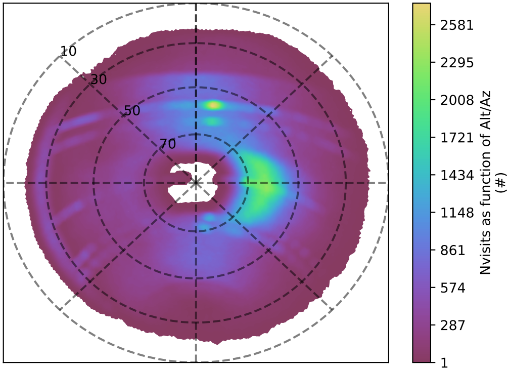
early_u_fpextra4.0_v3.4_10yrs r band: Nvisits as function of Alt/Az
