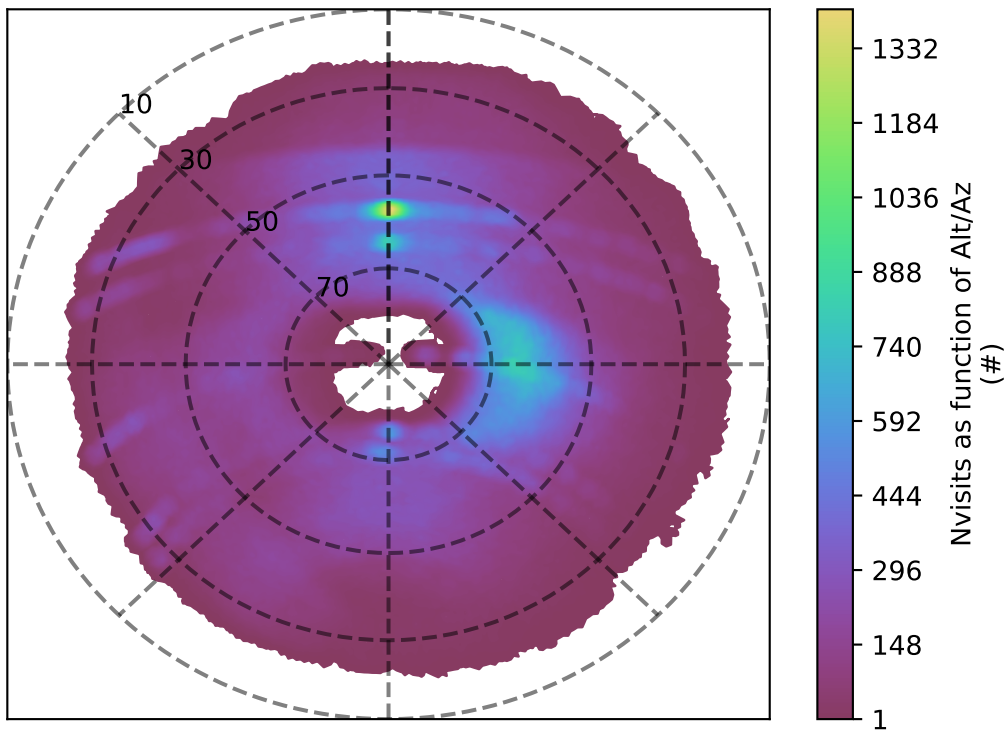
early_u_fpextra4.0_v3.4_10yrs g band: Nvisits as function of Alt/Az
