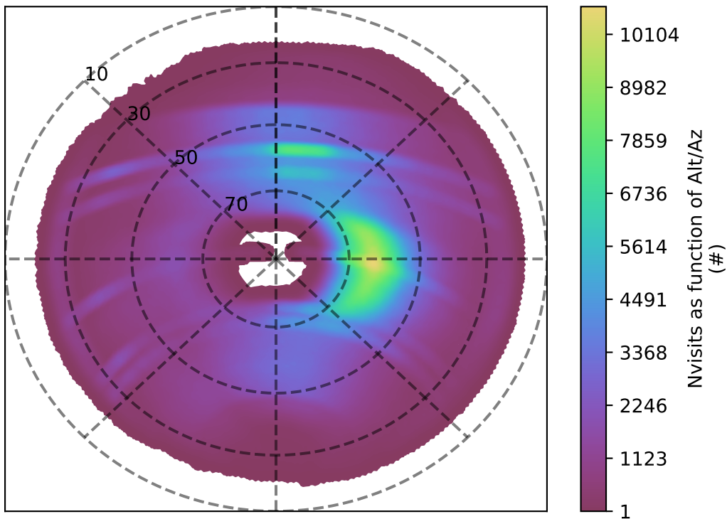
early_u_fpextra4.0_v3.4_10yrs all bands: Nvisits as function of Alt/Az
