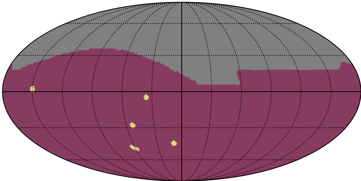
early_u_fpextra4.0_v3.4_10yrs All sky: NumberOfQuickRevisits
