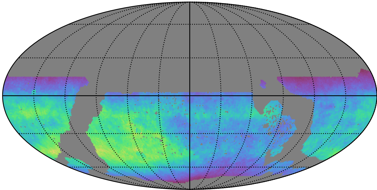
early_u_fpextra4.0_v3.4_10yrs WFD z band: Normalized Teff
