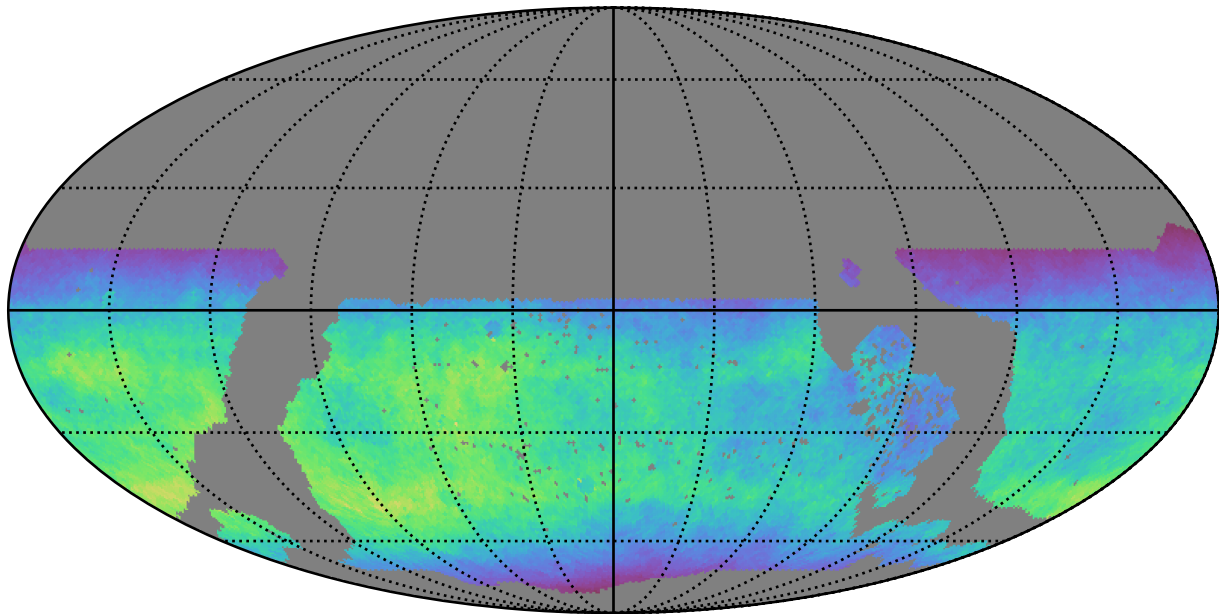
early_u_fpextra4.0_v3.4_10yrs WFD y band: Normalized Teff
