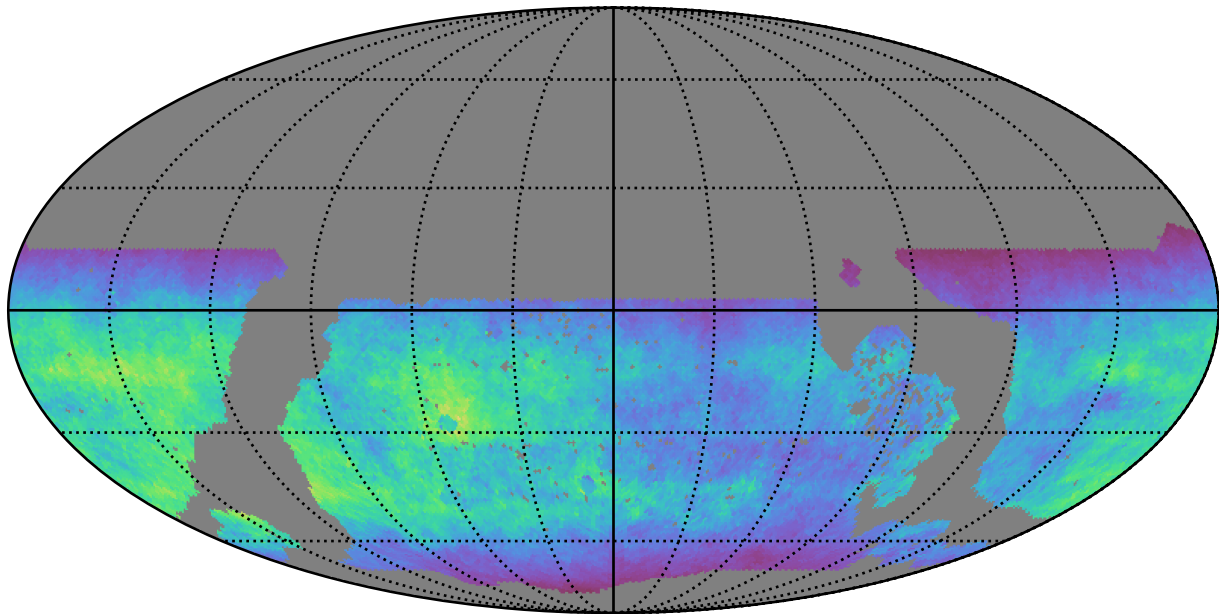
early_u_fpextra4.0_v3.4_10yrs WFD u band: Normalized Teff
