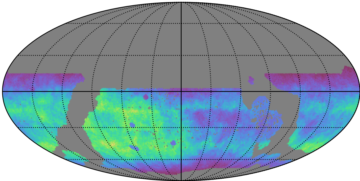
early_u_fpextra4.0_v3.4_10yrs WFD g band: Normalized Teff
