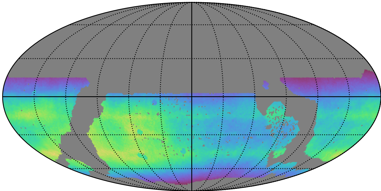
early_u_fpextra4.0_v3.4_10yrs WFD all bands: Normalized Teff
