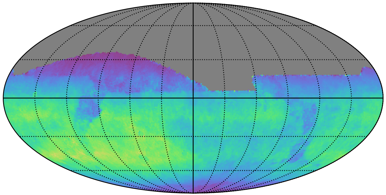
early_u_fpextra4.0_v3.4_10yrs All sky z band: Normalized Teff
