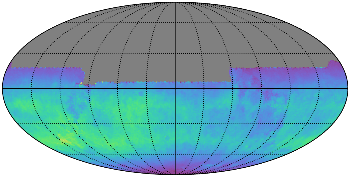
early_u_fpextra4.0_v3.4_10yrs All sky y band: Normalized Teff
