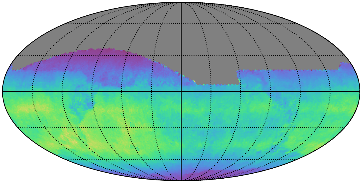
early_u_fpextra4.0_v3.4_10yrs All sky i band: Normalized Teff
