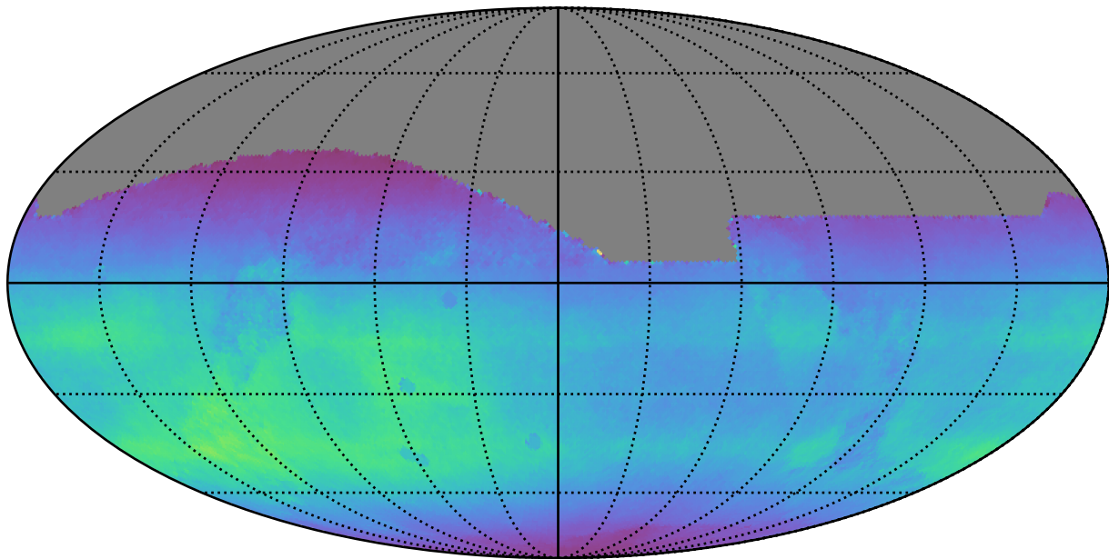
early_u_fpextra4.0_v3.4_10yrs All sky all bands: Normalized Teff
