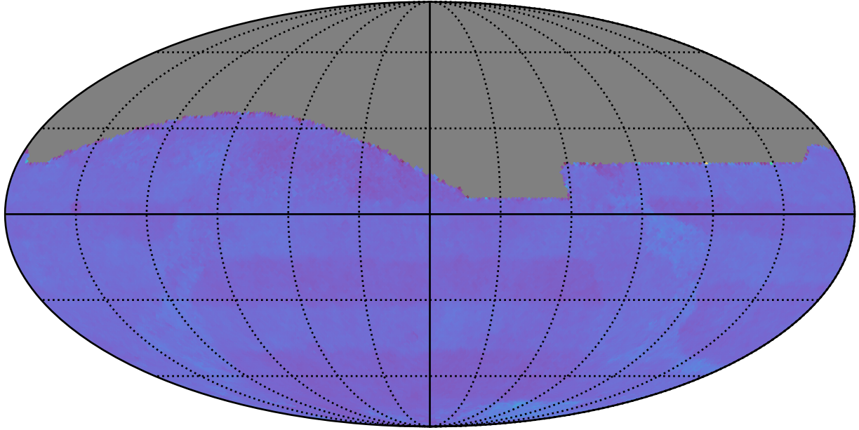
early_u_fpextra4.0_v3.4_10yrs All sky: Normalized Proper Motion Uncert @ 24.0
