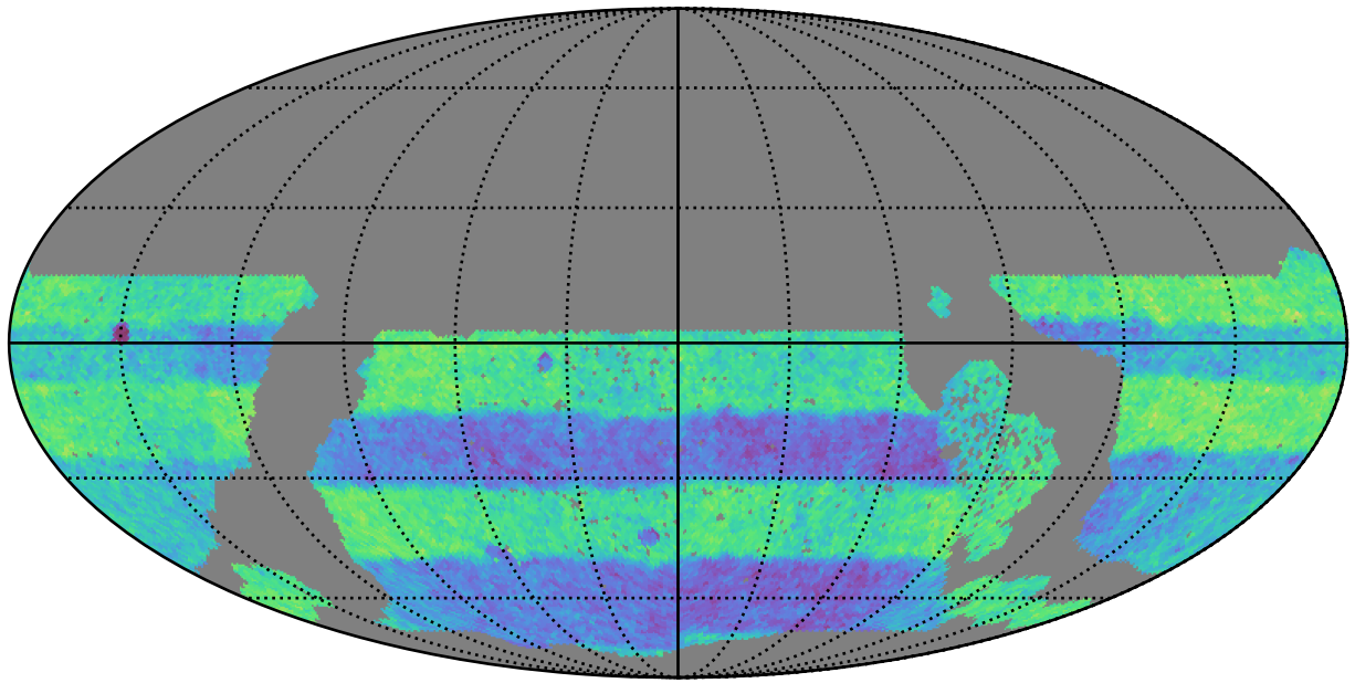
early_u_fpextra4.0_v3.4_10yrs WFD: Normalized Proper Motion Uncert @ 20.5
