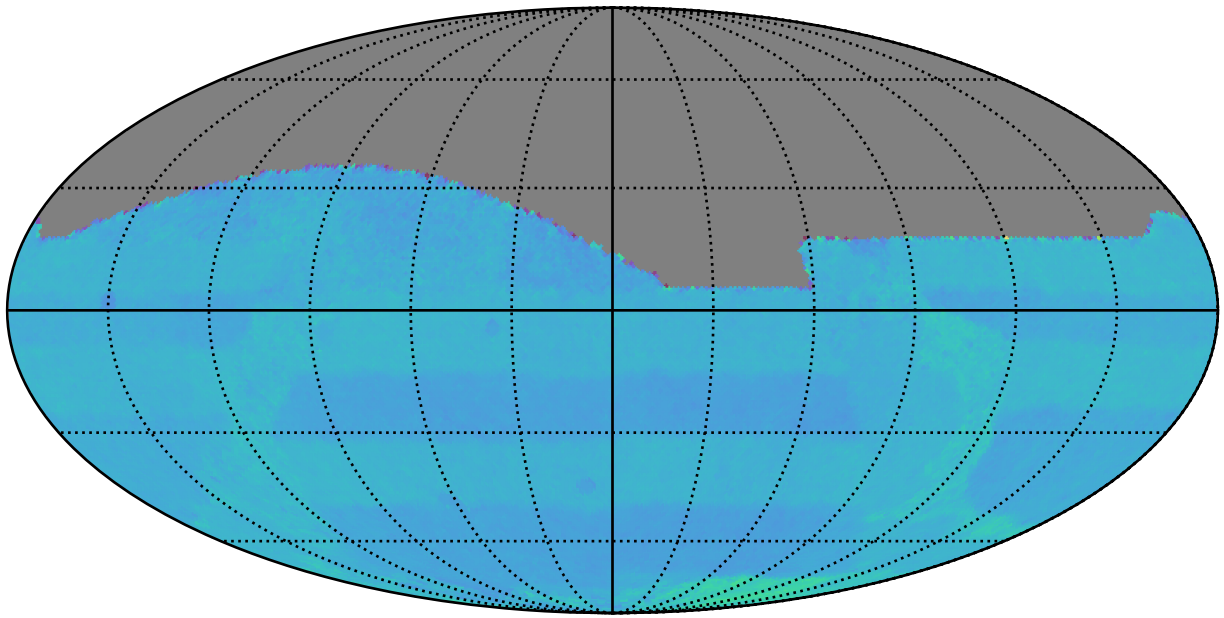
early_u_fpextra4.0_v3.4_10yrs All sky: Normalized Proper Motion Uncert @ 20.5
