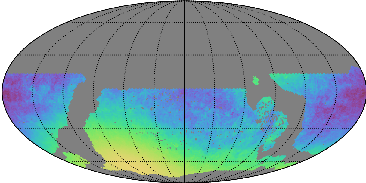
early_u_fpextra4.0_v3.4_10yrs WFD y band only: Normalized Parallax Uncert @ 21.3
