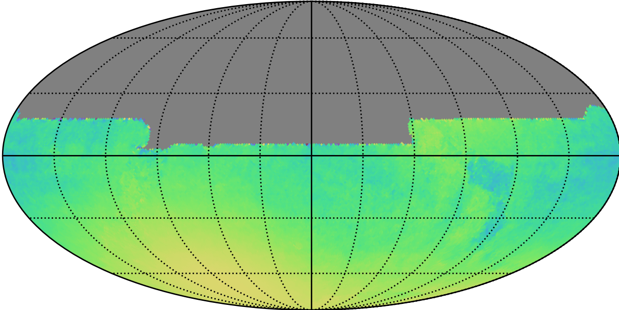
early_u_fpextra4.0_v3.4_10yrs All sky y band only: Normalized Parallax Uncert @ 21.3
