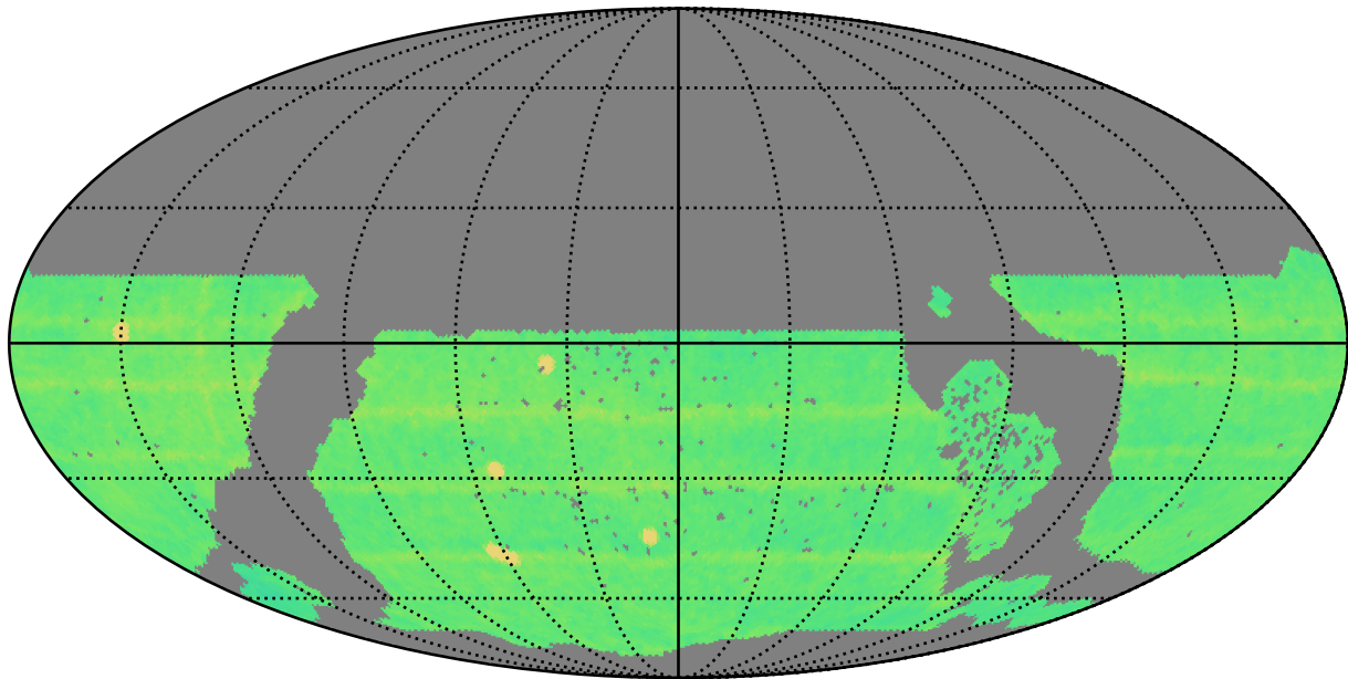
early_u_fpextra4.0_v3.4_10yrs WFD all bands: N Unique Nights
