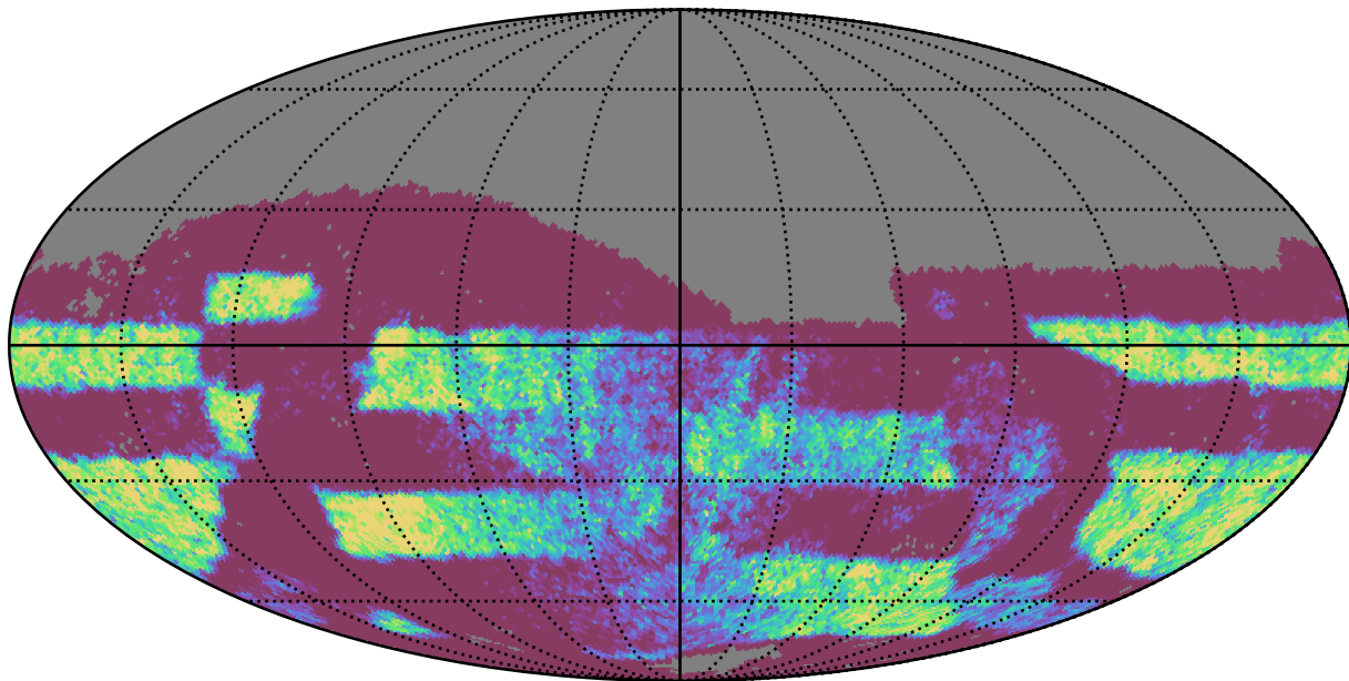
early_u_fpextra4.0_v3.4_10yrs Yr 3-4 z band: NVisits
