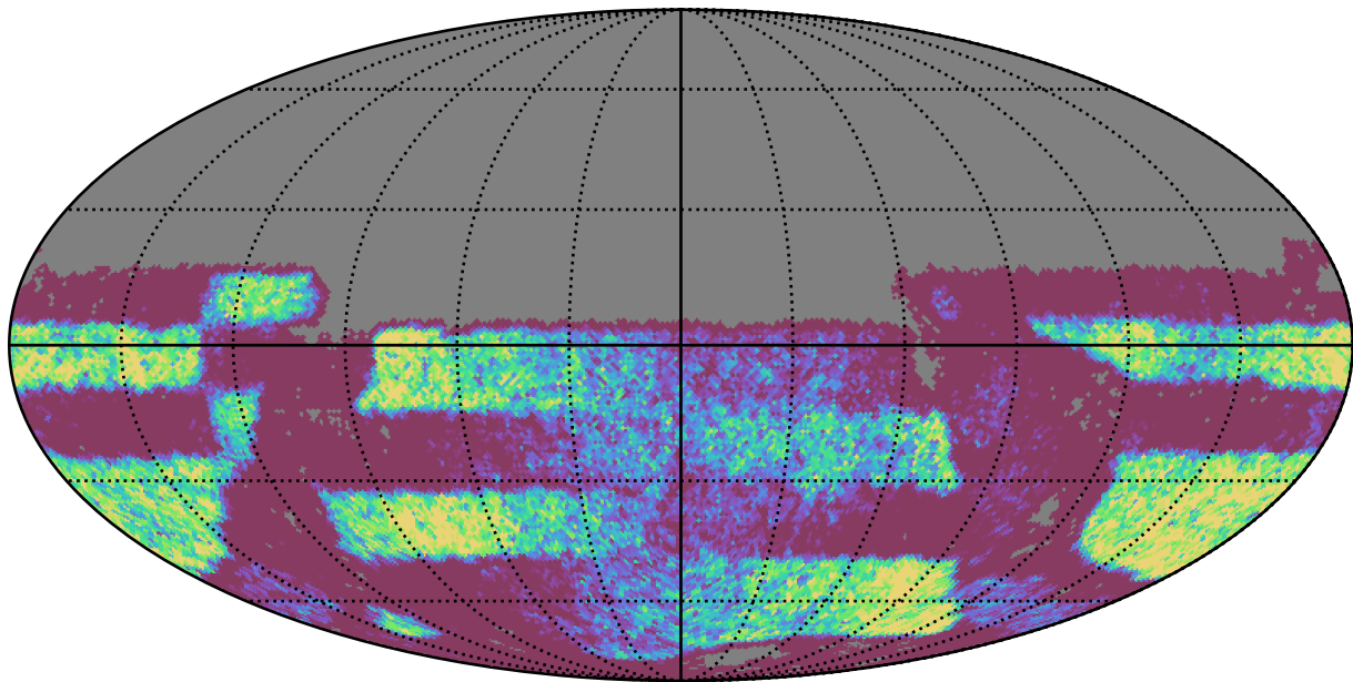
early_u_fpextra4.0_v3.4_10yrs Yr 3-4 y band: NVisits
