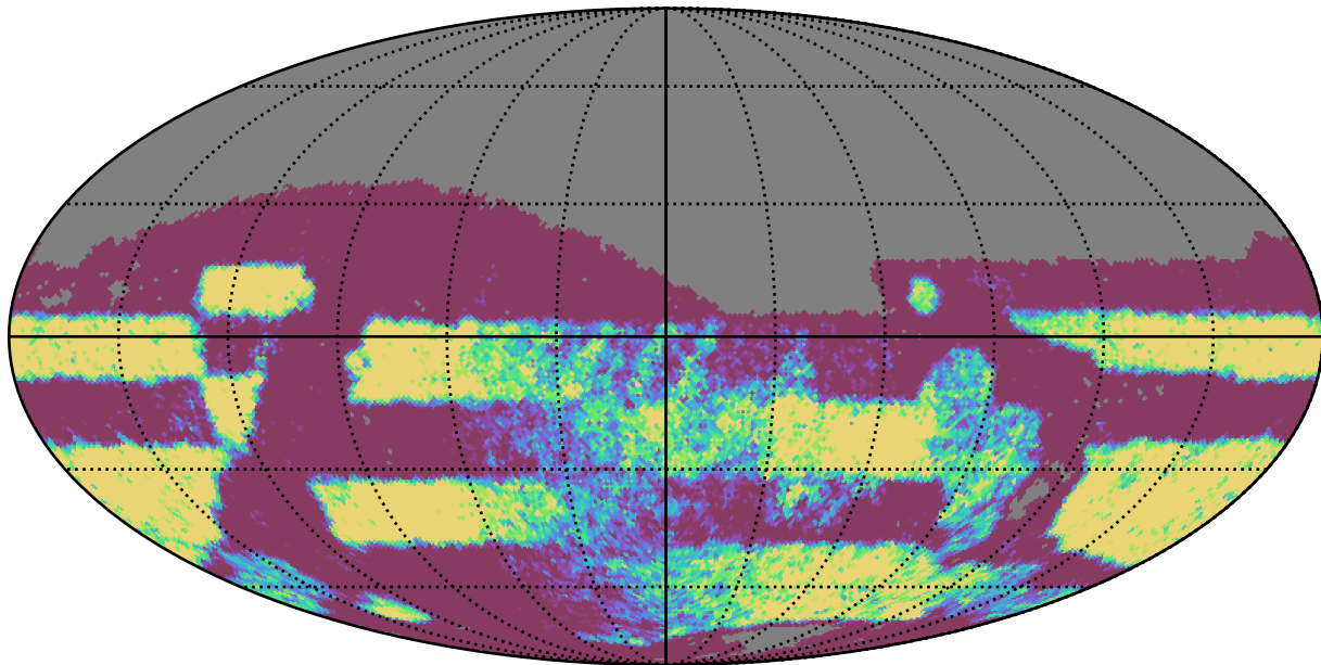
early_u_fpextra4.0_v3.4_10yrs Yr 3-4 r band: NVisits
