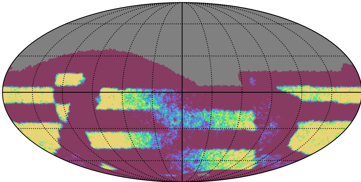
early_u_fpextra4.0_v3.4_10yrs Yr 3-4 all bands: NVisits
