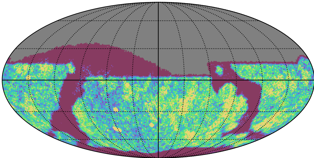
early_u_fpextra4.0_v3.4_10yrs Yr 1 i band: NVisits
